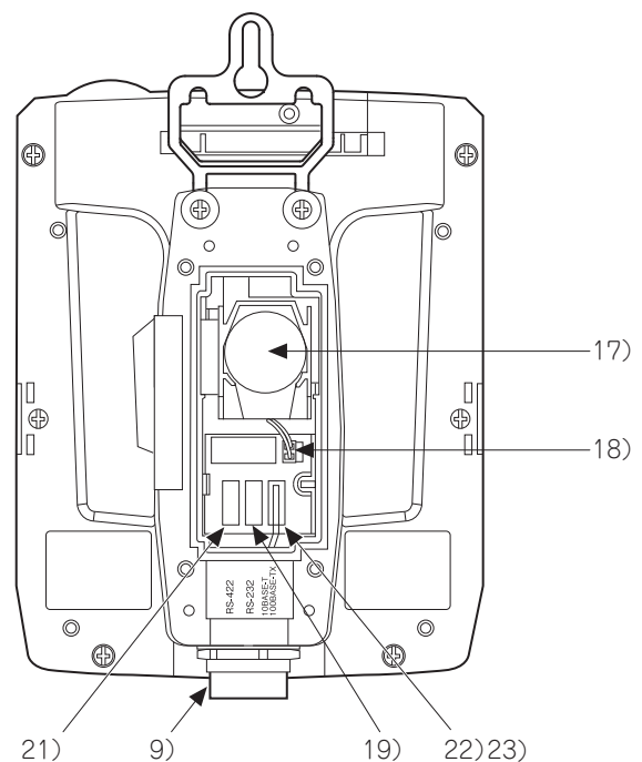
Environmental protection back cover opened
