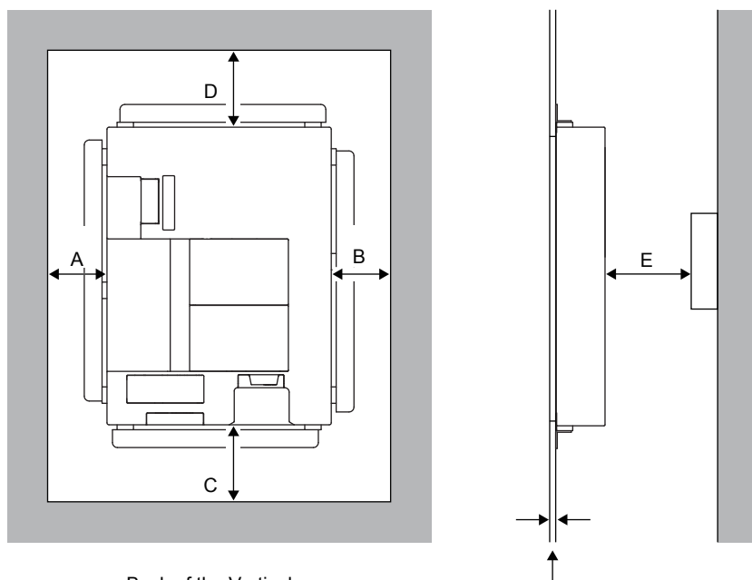
Back of the Vertical
