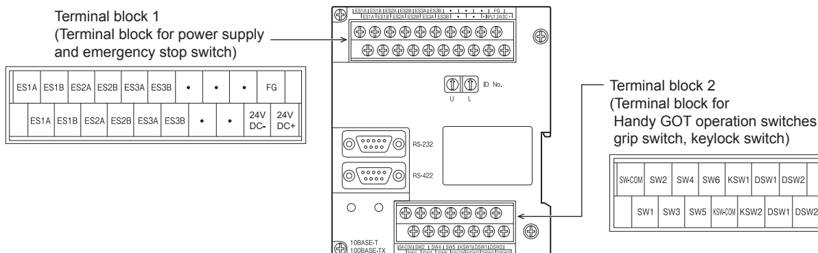
Terminal block 1
